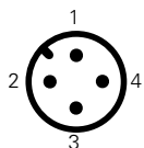
M12 connector, 4 poles
