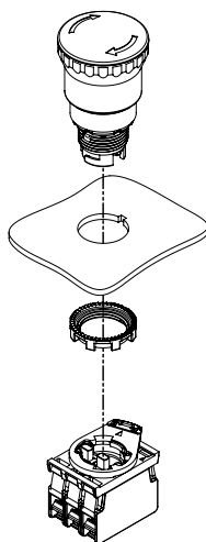
Alternative position contact block
